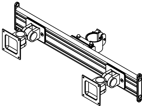
Assembled View
