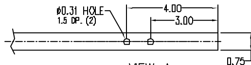
VIEW-A (M 4:1)
